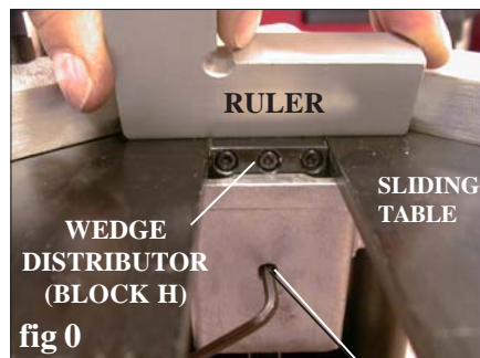
LOCKING SCREW
