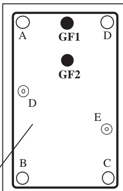
BLOC H SCREW POSITIONS
