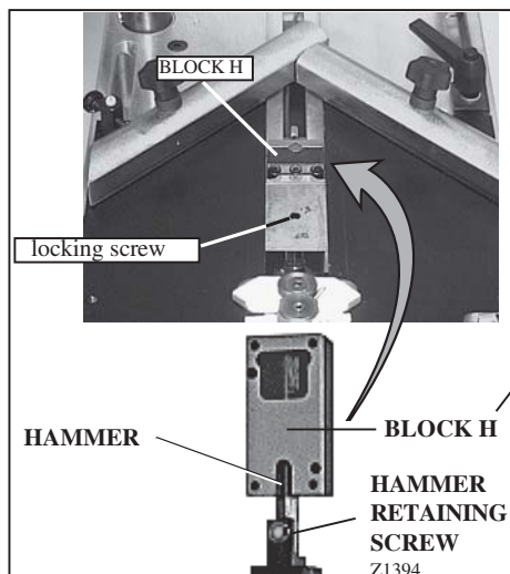
BLOC H SCREW POSITIONS
